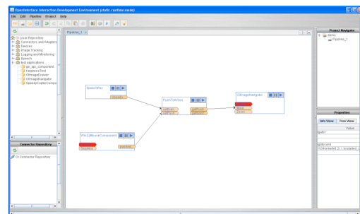
Figure 1. OIDE: a graphical editor for assembling components. (from [4])
